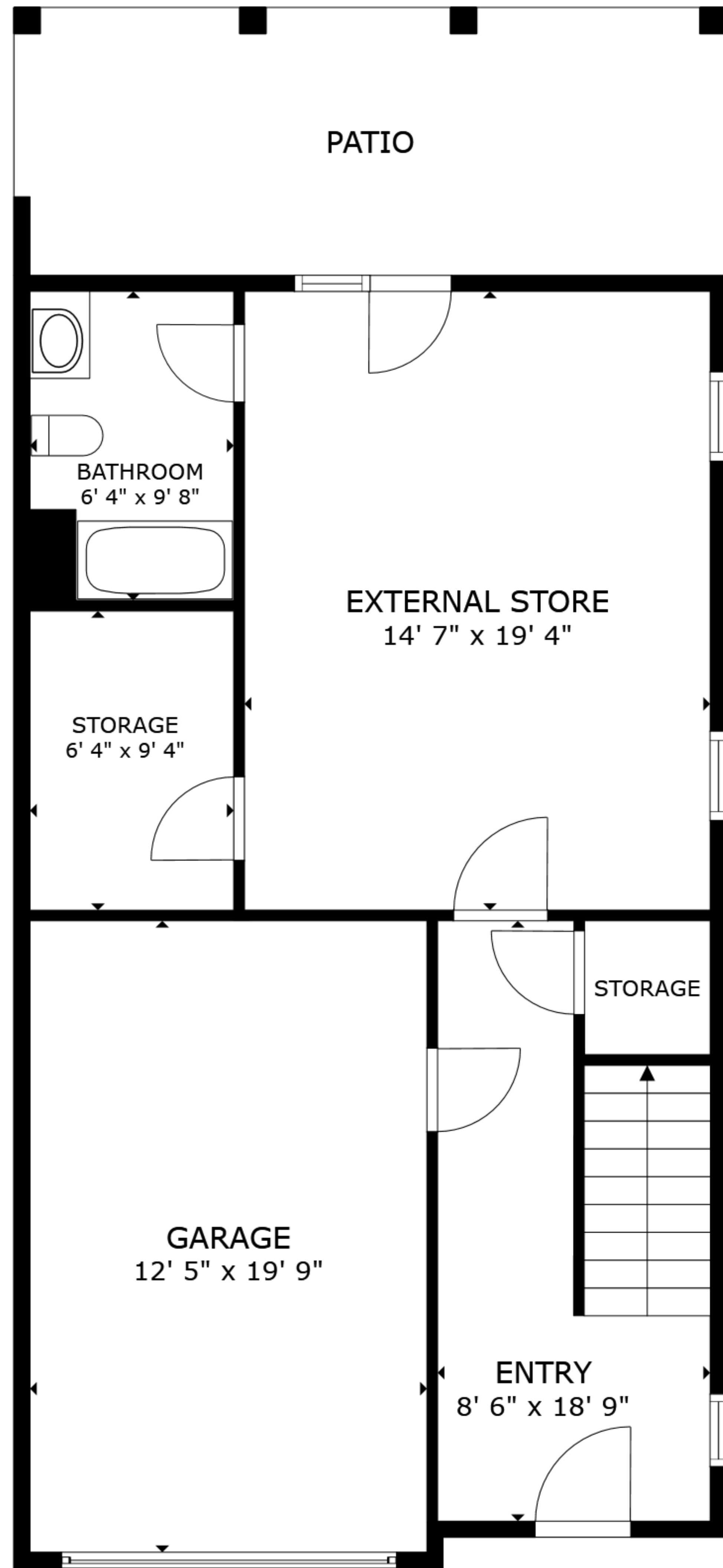
FLOOR 1
